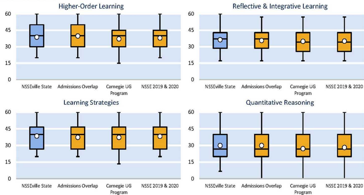
Score Distributions
