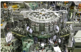
JT-60SA
