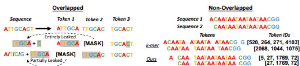
Figure 1: Illustration of the drawbacks of k-mer tokenization. In the overlapping setting, information about a masked token is leaked by its adjacent tokens, while in the non-overlapping setting, adding/deleting one nucleotide base leads to a dramatic change in the tokenized sequence.
