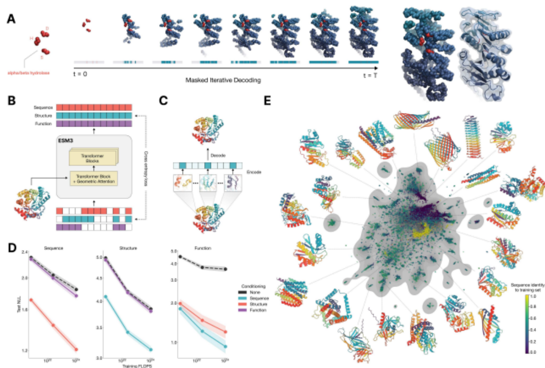
Figure 1. ESM3 is a generative language model that reasons over the sequence, structure, and function of proteins. (A) Iterative sampling with ESM3. Generation of an alpha/beta hydrolase. Sequence, structure, and function can all be used to prompt the model. At each timestep t , a fraction of the masked positions are sampled until all positions are unmasked. (B) ESM3 architecture. Sequence, structure, and function are represented as tracks of discrete tokens at the input and output. The model is a series of transformer blocks, where all tracks are fused within a single latent space; geometric attention in the first block allows conditioning on atomic coordinates. ESM3 is supervised to predict masked tokens. (C) Structure tokenization. Local atomic structure around each amino acid is encoded into tokens. (D) Models are trained at three scales: 1.4B, 7B, and 98B parameters. Negative log likelihood on test set as a function of training FLOPs shows response to conditioning on each of the input tracks, improving with increasing FLOPs. (E) Unconditional generations from ESM3 98B (colored by sequence identity to the nearest sequence in the training set), embedded by ESM3, and projected by UMAP alongside randomly sampled sequences from UniProt (in gray). Generations are diverse, high quality, and cover the distribution of natural sequences.
