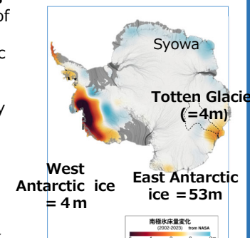
Figure 2. Antarctic ice mass and its recent change
