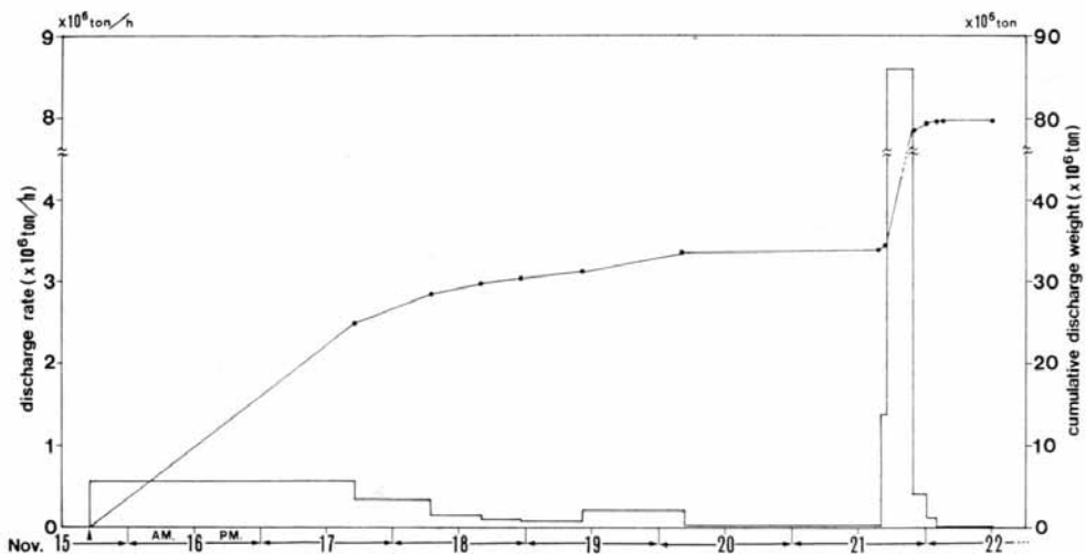
Fig. 14. Changes in magma discharge rate and cumulative discharge weight during the 1986 Izu-Oshima eruption.
