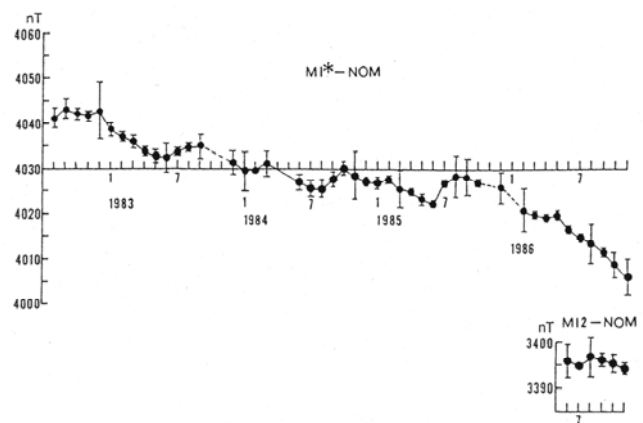
Fig. 5. Time variations in total intensity at MI2* in comparison with those at MI*.
