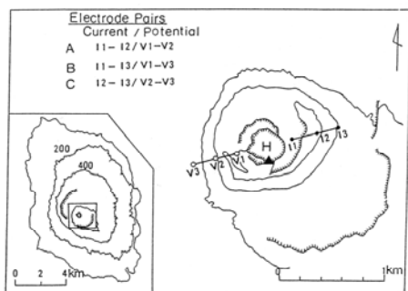
Fig. 3. Electrode arrangements of bipole-bipole measurements across the central crater. Three pairs of electrodes are used for monitoring the resistivity change: A with the current electrodes I 1 , I 2 and the potential electrodes V 1 , V 2 ; B with I 1 , I 3 and V 1 , V 3 ; C with I 2 , I 3 and V 2 , V 3 . The solid triangle designates the newly formed crater from which the central eruptions occurred in 1986–1987. H represents the crater pit which was filled with lava from the new crater shown by the double circle.
