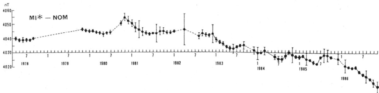
Fig. 3. Time variation in total intensity difference between MI* and NOM.
