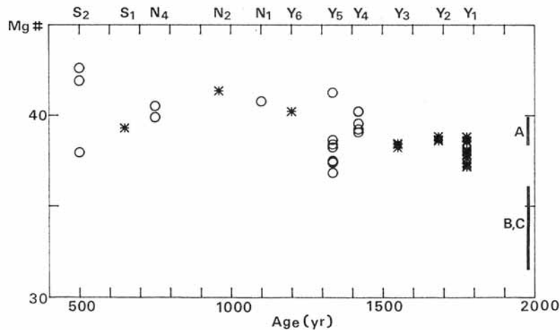
Fig. 16. Chronological variation of Mg# of lavas and ejecta. Circle: major eruption with flank eruption, Asterisk: major eruption without flank eruption. The abbreviations for the major eruptions (NAKAMURA, 1964) are shown at the top.
