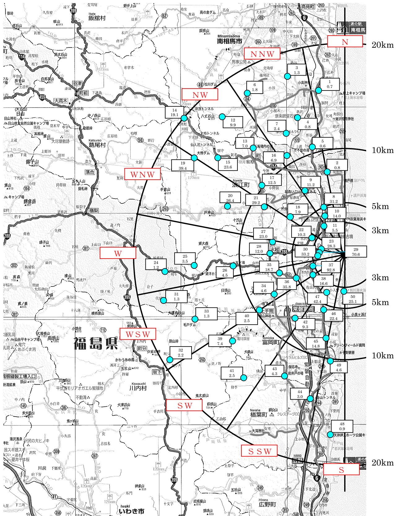
Readings of Radioactivity Concentration of Nuclides in the Air inside of the 20 km Zone of Fukushima Dai-ichi NPP
