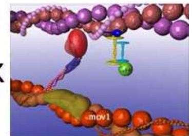
CafeMol
