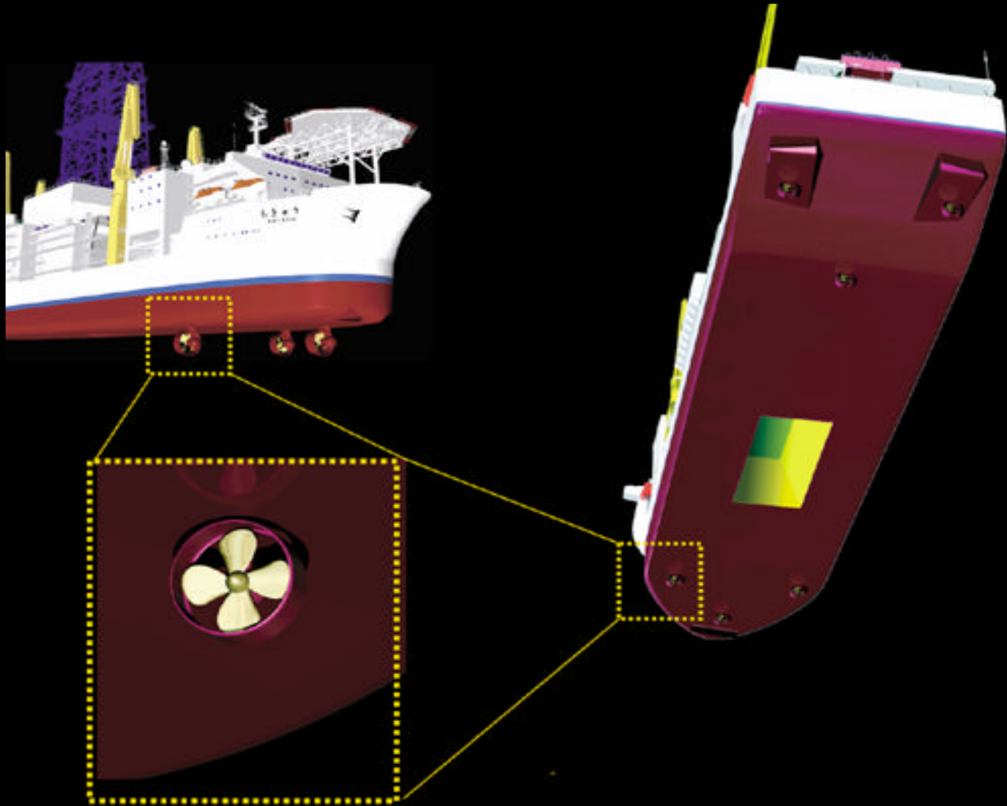
Azimuth thruster
