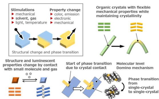
Fig. 1. Soft Crystals: features and examples of flexible new materials with high order.
