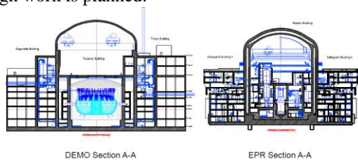
Fig. 4: DEMO Tokamak Building Complex (compared with EPR)
