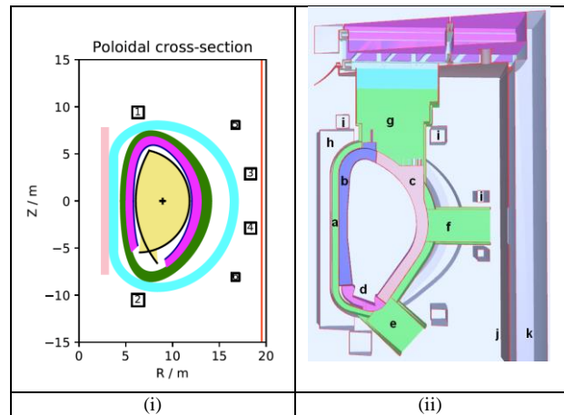
Fig. 3: (i) Elevation view of the tokamak as generated by PROCESS; (ii) Tokamak radial-build: a) vacuum-vessel; breeding blanket (inboard); c) breeding blanket (outboard); d) divertor; e) lower port; f) (equatorial port); g) upper port; h) toroidal field coils; i) poloidal field coils; j) cryostat; k) bioshield
