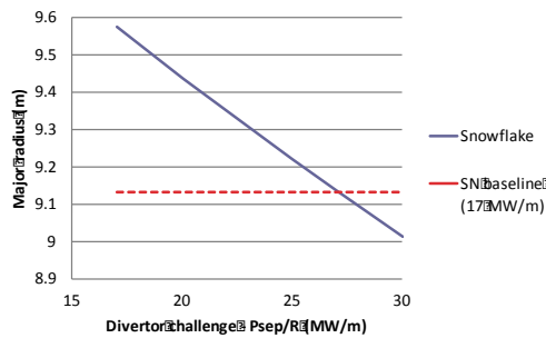
Figure 5: Plot showing major radius as a function of divertor physics performance (quantified as P_{sep}/R ) for a snowflake divertor device targeting 500MWe and a 2 h pulse length, taking magnet design, plasma performance, and additional space requirements into account. The dotted red line is the size of the ITER-like baseline design.
